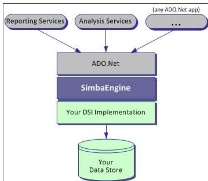
Figure 1: High-level view of Simba SDK
